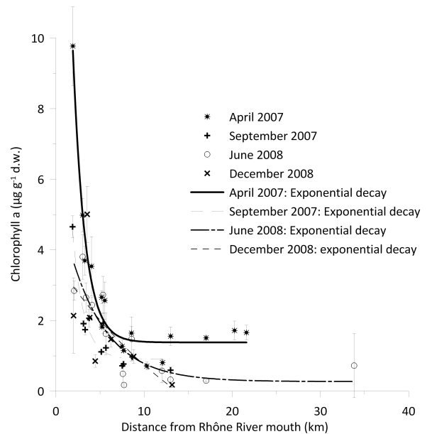
Fig. 5. Surface sediments Chl a contents as a function of distance from the river outlet: \star April 2007, \blackplus September 2007, \circ June 2008 and \times December 2008.
