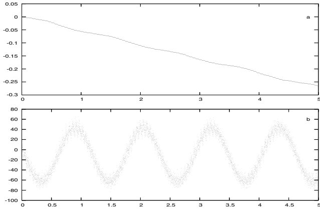
Figure 6. Study of the critical angle of the resonance 4g - g_5 + \nu_{2,5} = 0 . Top panel: Naïve candidate of critical angle. 4\varpi - \varpi_5 + 2\lambda_5 - 5\lambda_6 (in millions of degrees) versus time (in Myr). Bottom panel: actual critical angle. Argument of \hat{z}^4 \exp(i(\nu_{2,5} - g_5)t) in degrees versus time.
