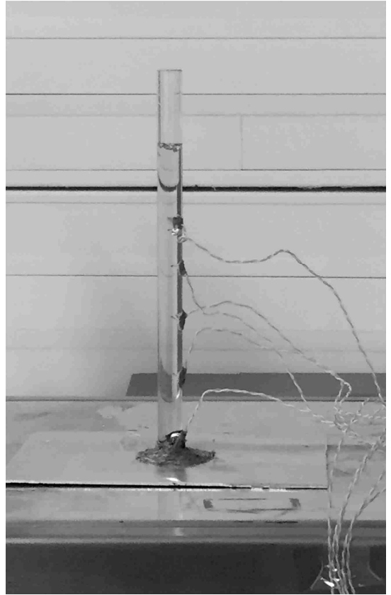
Fig. 3. Experimental setup
