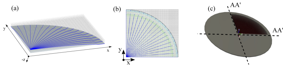
Fig. 11. (a) 3D view of the imported splines over the K \times K matrix of posts of equal heights, (b) 2D splines representation over the K \times K matrix, (c) final modulated metal posts over the bottom metal plate of the PPW.
