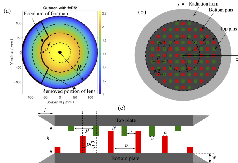
Fig. 1. (a) Effective refractive index n_{eff} of the Gutman Lens with focal arc f = R/2 , (b) PPW GRIN Gutman lens layout using an IGS unit cell (top view), (c) 2D cut view, p=2.4 , a=0.8 , s=0.4 , h'=1.9 , h=4 , w=12 , all dimensions in mm.
