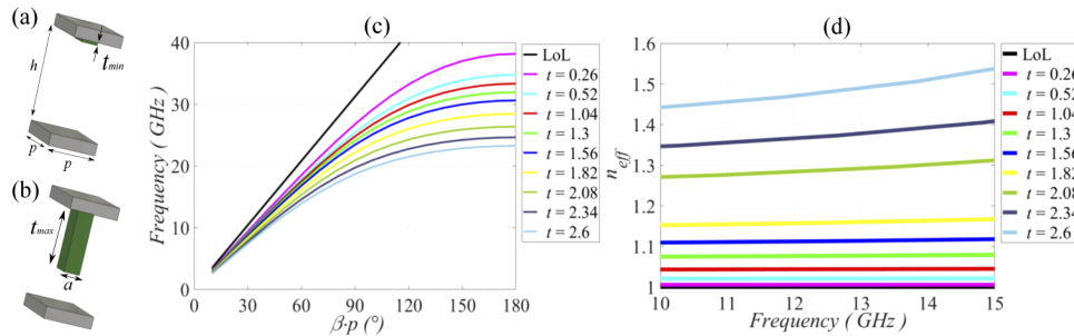
Fig. 2. (a) LoL propagation (b) fakir unit cell - first DoF (c) dispersion and (d) effective index values.
