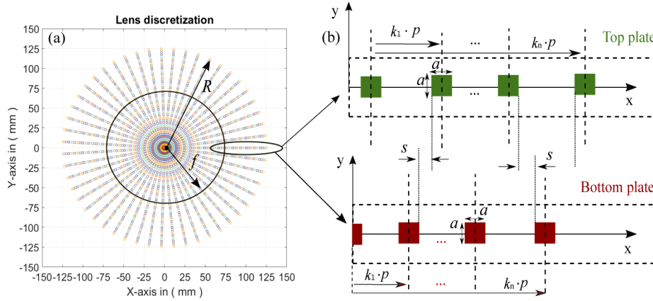
Fig. 6. (a) Lens discretization, (b) K discretized values of the bottom and top metal posts.
