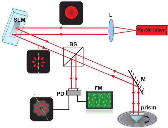
FIG. 1. Experimental setup: the fundamental mode of a He-Ne laser (wavelength \lambda = 633 nm) is converted to a superposition of LG beams of opposite charges using a Spatial Light Modulator (SLM). The beam impinges on a rotating right angle prism. The retro reflected light is sent to a screen or to a photodiode connected to a frequency meter (FM). L: lens, BS: beam splitter, M: mirror, and PD: photodiode.
