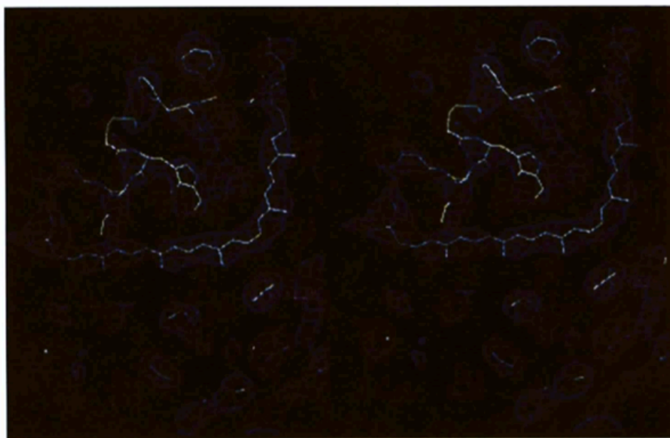
Fig. 6. Stereoview of the 2F_o - F_c electron-density map for the spheroidene molecule.
