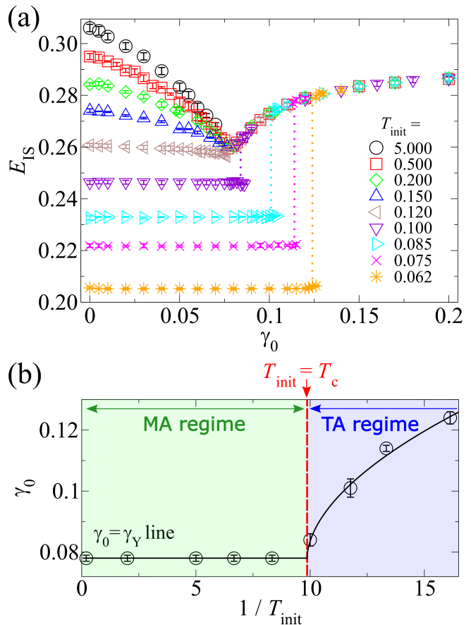
FIG. 2. (a) Steady-state inherent structure energy E_{\text{IS}} as a function of the strain amplitude \gamma_0 for several T_{\text{init}} . The dashed vertical lines represent the discontinuous jumps. (b) Nonequilibrium phase diagram in the (\gamma_0, T_{\text{init}}^{-1}) plane. The critical temperature T_c (red long dashed line) divides the phase space into the mechanical annealing (MA) and thermal annealing (TA) regimes. The black solid line separates the elastic and yielded regions (see the text).
