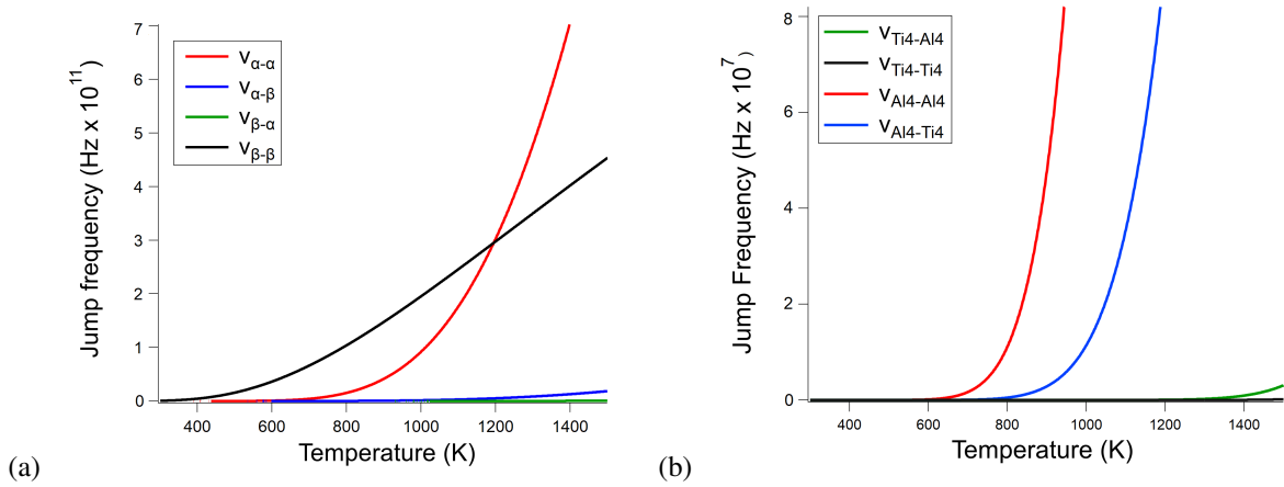
Figure 9: Jumping rates as a function of temperature: (a) oxygen, (b) boron. For simplicity, the octahedral sites are identified with the most abundant element, i.e. A/4 indicates the [Ti_2Al_4] octahedron.
