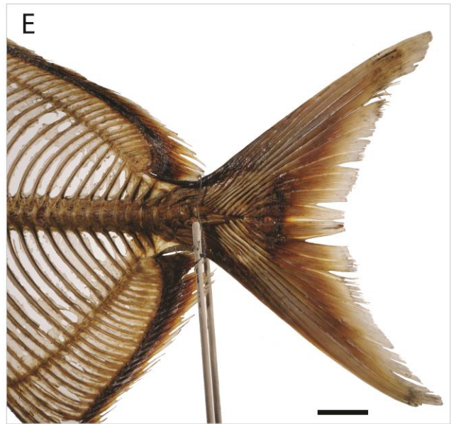
Figure 3. Caudal skeleton of several studied taxa. A, † Aipichthys minor (reconstruction), after Patterson (1968: fig. 11A). Scale bar: 1 mm. B, † Aspesaipichthys cavaensis (reconstruction), after Taverne (2004: fig. 7). Scale bar: 1 mm. C, Velifer hypselopterus (= V. africanus ) (Veliferidae), after Oelschläger (1983: Fig. 82). Scale bar: 1 mm. D, † Aipichthys velifer , MNHN.F.HAK57, showing hypurostegy of the caudal fin rays. Scale bar: 5 mm. Photo D. Davesne. E, Lampris guttatus , ZMUC 74, showing hypurostegy of the caudal fin rays. Scale bar: 5 cm. Photo M.A. Krag. Abbreviations: hy, hypural; phy, parhypural; pu, preural vertebral centrum; u, ural vertebral centrum.
