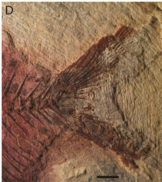
Figure 3. Caudal skeleton of several studied taxa. A, † Aipichthys minor (reconstruction), after Patterson (1968: fig. 11A). Scale bar: 1 mm. B, † Aspesaipichthys cavaensis (reconstruction), after Taverne (2004: fig. 7). Scale bar: 1 mm. C, Velifer hypselopterus (= V. africanus ) (Veliferidae), after Oelschläger (1983: Fig. 82). Scale bar: 1 mm. D, † Aipichthys velifer , MNHN.F.HAK57, showing hypurostegy of the caudal fin rays. Scale bar: 5 mm. Photo D. Davesne. E, Lampris guttatus , ZMUC 74, showing hypurostegy of the caudal fin rays. Scale bar: 5 cm. Photo M.A. Krag. Abbreviations: hy, hypural; phy, parhypural; pu, preural vertebral centrum; u, ural vertebral centrum.
