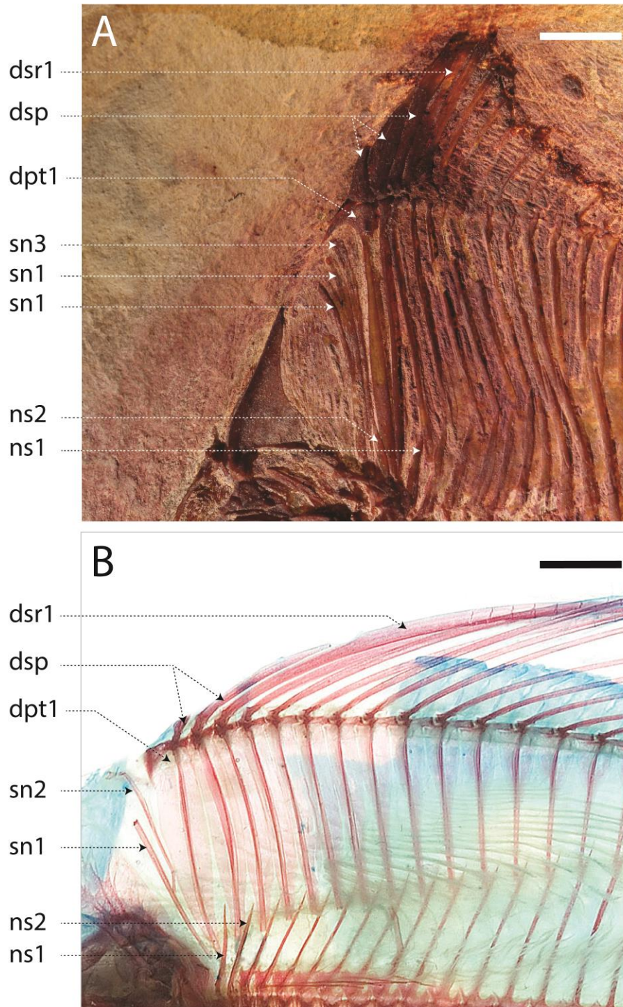
Figure 2. Dorsal fin skeleton of two studied taxa. A, †Aipichthys velifer , MNHN.F.HAK57. Scale bar: 1 cm. Photo D. Davesne. B, Velifer hypselopterus (Veliferidae), AMS 21840020. Scale bar: 5 mm. Photo courtesy D. Johnson. Abbreviations: dpt, dorsal pterygiophore; dsp, dorsal spine; dsr, dorsal soft ray; ns, neural spine; sn, supraneural.
