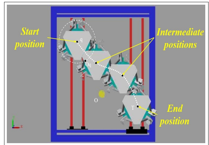
Fig. 8. Platform navigation to the right of the obstacle in SimMechanics
