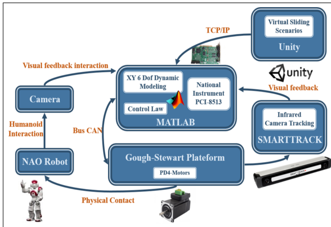
Fig. 3. Technological mechatronics architecture
