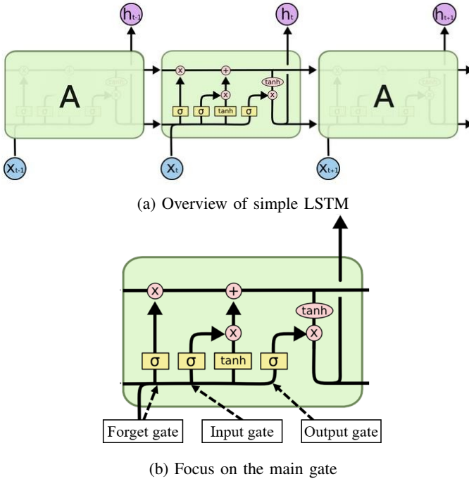
Fig. 5: Architecture of LSTM from [37]
