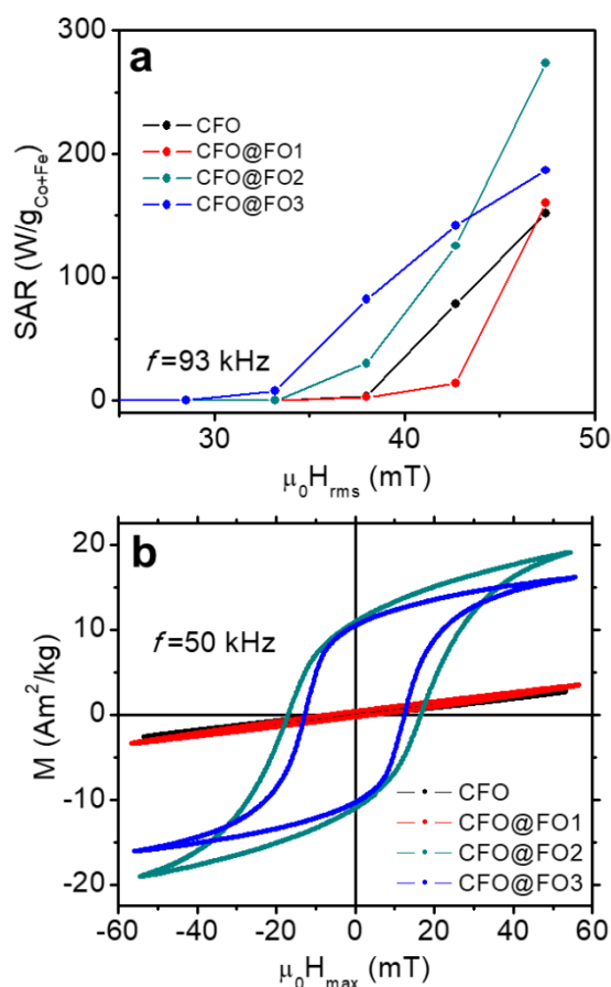
Figure 4. SAR values measured by calorimetry at a frequency of 93 kHz (a) and high-frequency hysteresis loops at 50 kHz (b) at room temperature for the Co 0.6 Fe 2.4 O 4 samples with different Fe 3 O 4 shell thickness.
