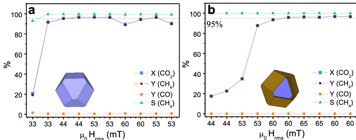
Figure 5. Percentage of CO 2 conversion, CH 4 and CO yields and CH 4 selectivity as a function of \mu_0 H_{rms} for CFO/Ni/S (a) and for CFO@FO 2 /Ni/S systems (b). Sketches in blue and in blue-brown represent the single Co 0.6 Fe 2.4 O 4 phase and the core-shell Co 0.6 Fe 2.4 O 4 @Fe 3 O 4 cuboctahedron employed for the heating, respectively. Dashed lines indicate the 95 % level.
