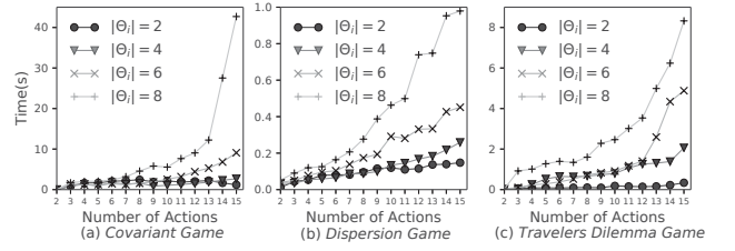
Figure 1. Avg. execution time of MILP (s), n = 2
