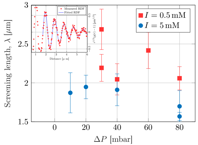
Fig. 7 Screening length as a function of applied pressure drop for the two different ionic strengths. Error bars correspond to fit’s 95%-confidence bounds. Inset: normalized RDF for \Delta P = 80 \text{ mbar} and I = 0.5 \text{ mM} . The solid line represents the fit obtained with equation 8.
