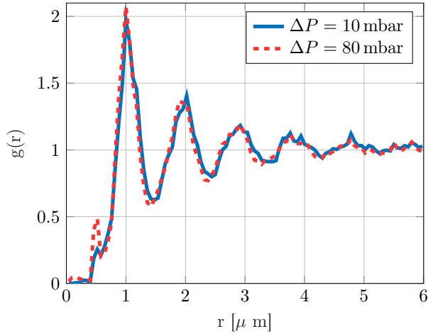
Fig. 6 Radial distribution function for two applied pressure drops at I = 5 \text{ mM} . The blip observed at r = 0.5 \mu\text{m} is probably related to aliasing.
