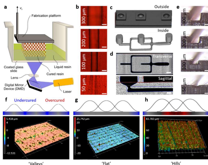
Fig. 1. High-resolution stereolithographic 3D printing of microfluidic channels. (a) Schematic representation of stereolithography with a digital micromirror device (DMD), which was used to manufacture (b) microfluidic channels made of PIC100 resin. Scale bars indicate 100 \mu\text{m} . The designed (i.e., intended) channel widths are indicated per microphotograph with white text. (c) 3D reconstructed \mu\text{CT} data of printed microfluidic device. (d) Cross-sectional \mu\text{CT} images were digitally overlapped with its original CAD design (blue lines) and confirmed high 3D print fidelity. Scale bar transverse plane indicates 500 \mu\text{m} . Scale bar sagittal plane indicates 150 \mu\text{m} . (e) Stereomicroscopic images of open-top channels confirmed accurate inter-layer alignment. Scale bar indicates 300 \mu\text{m} . (f-h) Laser-scanned surface roughness of the 3D printed channels as determined by confocal profilometry. Voxel undercuring and overcuring resulted in apparent 'valleys' and 'hills' at the voxels' intersection, respectively.
