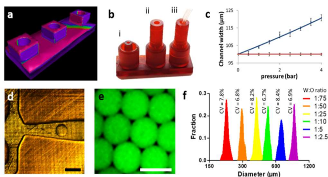
Fig. 2. Microdroplet production using a 3D printed microfluidic device. (a) Stereolithographic printing enabled the printing of a microfluidic droplet generator that could be readily provided with (b) Luer-Lok type connectors, which enable swift chip-to-world connections as visualized by a (i) male Luer-Lok connector, (ii) that can be locked to a separately printed female Luer-Lok, (iii) through which microfluidic tubing can be connected. (c) Channel width (average \pm standard deviation; n = 3 ) analysis as a function of internal pressure revealed nihil pressure-induced deformation of 3D printed channels (red curve) as compared to conventional PDMS-on-glass channels (blue curve) with identical designs. (d) Microphotograph of water-in-oil droplet generation using a 3D printed microfluidic device with a 150 \mu\text{m} wide nozzle confirmed chip functionality as well as the transparent nature of the photocured PIC100 resin allowing for on-chip monitoring using light microscopy. (e) Emulsified aqueous droplets containing fluorescein could be collected and imaged off-chip. (f) Size distribution and coefficient of variation (CV) of microdroplets ( n \geq 100 ) produced using 3D printed microfluidic device using various water / oil flow ratios (total flow rate 200 \mu\text{l}/\text{min} ). All scale bars indicate 200 \mu\text{m} .
