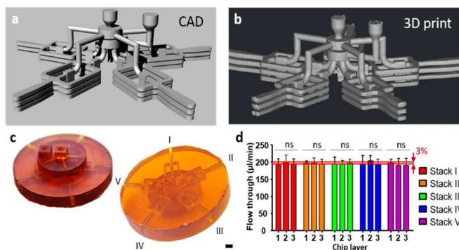
Fig 4. Printed 3D parallelized microfluidic device containing radially organized microdroplet generator stacks. (a) CAD design and (b) 3D reconstructed \mu CT data of the printed 3D parallelized microfluidic droplet generator device containing five radially organized stacks that each contain three droplet generators. (c) Photographs of a printed 3D parallelized microfluidic device from the top and bottom view. (d) The measured flow throughs (average \pm standard deviation; n = 3 ) of fifteen 3D parallelized droplet generators. 'ns' indicates p > 0.05 ; one-way ANOVA. Scale bar indicates 200 \mu m.
