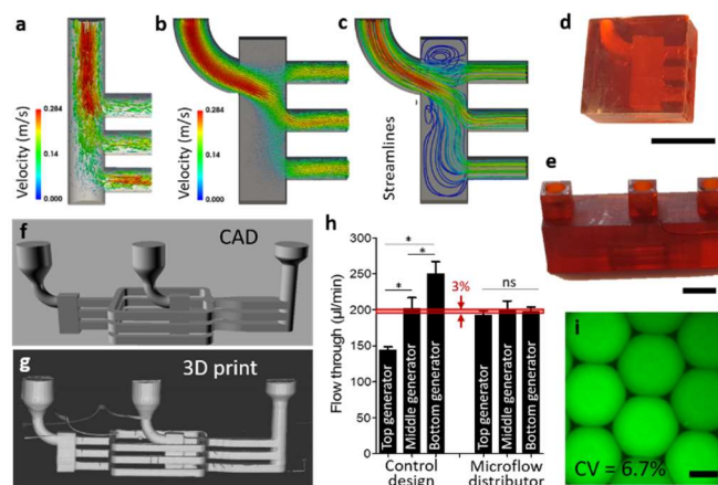
Fig. 3. Design and optimization of 3D printed stacked microfluidic droplet generator. (a) Numerical flow simulations of conventionally stacked microfluidic channels and (b,c) stacked channels connected via a computationally optimized microflow distributor. (d) Photographs of a 3D printed optimized microflow distributor and (e) a one-piece 3D printed microfluidic device containing a microflow distributors serially connected to three stacked droplet generators. Scale bars indicate 500 \mu\text{m} . Printing fidelity was investigated by comparing the (f) CAD design to (g) 3D reconstructed \mu\text{CT} data of the printed microdevice. (h) The measured flow throughs (average \pm standard deviation; n = 3 ) of conventionally stacked droplet generators (i.e., control design) and stacked droplet generators connected via the computationally designed microflow distributor. ‘*’ indicates p < 0.05 ; ‘ns’ indicates p > 0.05 ; one-way ANOVA. (i) Microphotograph of monodisperse (CV < 10%; n \geq 100 ) fluorescein containing aqueous microdroplets in oil that were produced using stacked microfluidic droplet generators containing a microflow distributor. Scale bar indicates 100 \mu\text{m} .
