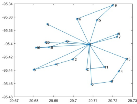
(b1) The 1 st stage paths in separated strategy with 20% increase of u_i and b_i
