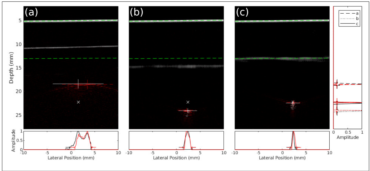
FIG. 4. US (grayscale) and PA (red overlay) images reconstructed using (a) DAS assuming a constant wavespeed of V_{water}=1486 \text{ m s}^{-1} and refraction-corrected imaging with a (b) layered medium including a bone layer with isotropic elasticity and (c) layered medium including a bone layer with anisotropic elasticity. The interfaces segmented in the US image using the method in (c) are shown with a dotted green line on all three panels. The true location of the top of the target is marked 'X'. Cross-sections along the lateral and depth direction are extracted at the point in the PA (dotted red lines) and US (white lines) images corresponding to the top of the target. The PA and US cross sections are shown in red and black, respectively. The width at -10 \text{ dB} of each cross section is denoted with arrows.
