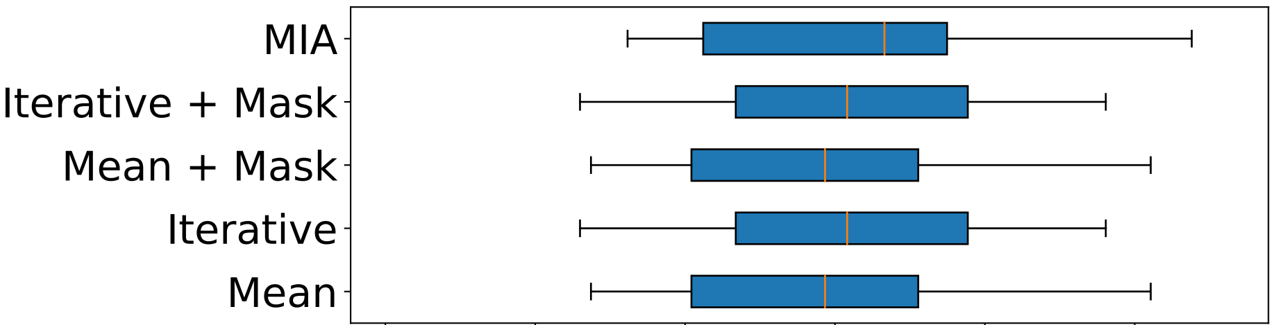
HGBoost MCAR
