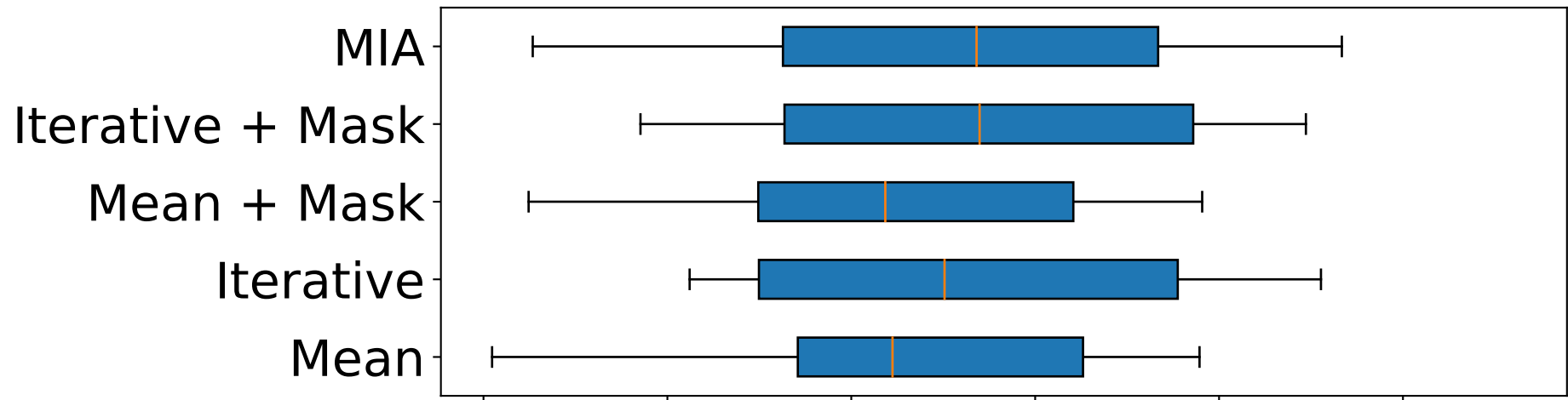
RandomForest MNAR
