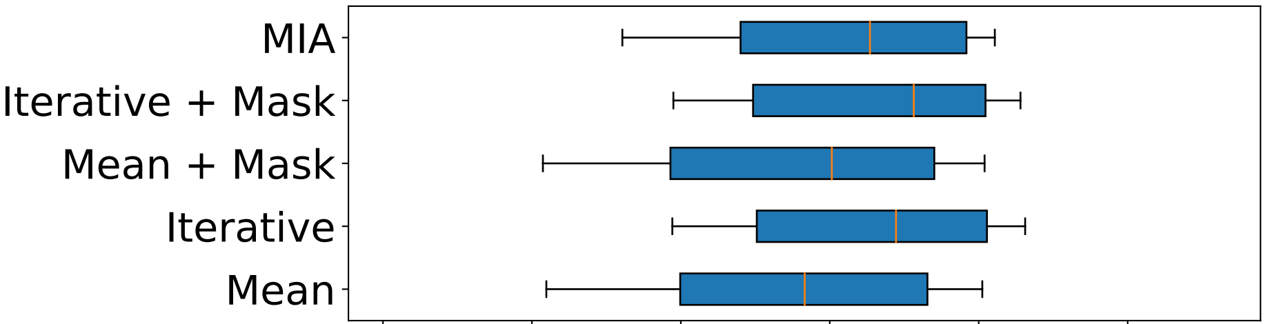
RandomForest MCAR
