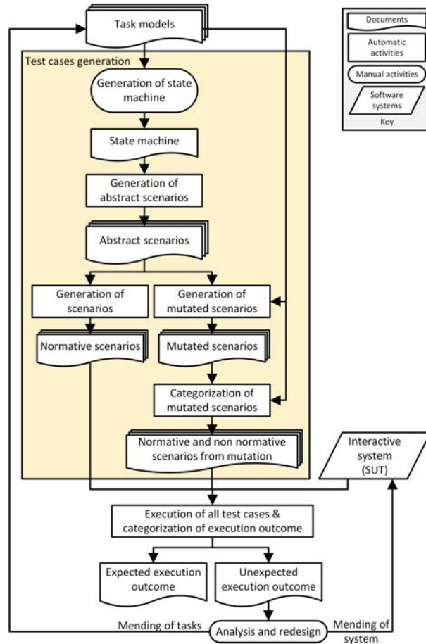
Fig. 1. Scenario-based testing of interactive applications process
