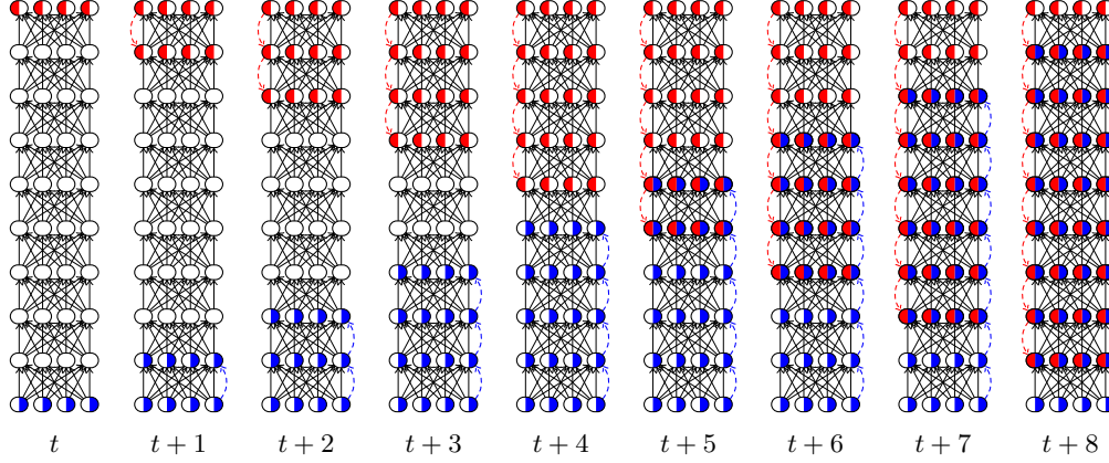
Figure 1: Forward and backward waves on a ten-level network when the input and the supervision are kept constant. When selecting a certain frame—defined by the time index—the gradient can consistently be computed by Backpropagation on “red-blue neurons”.
