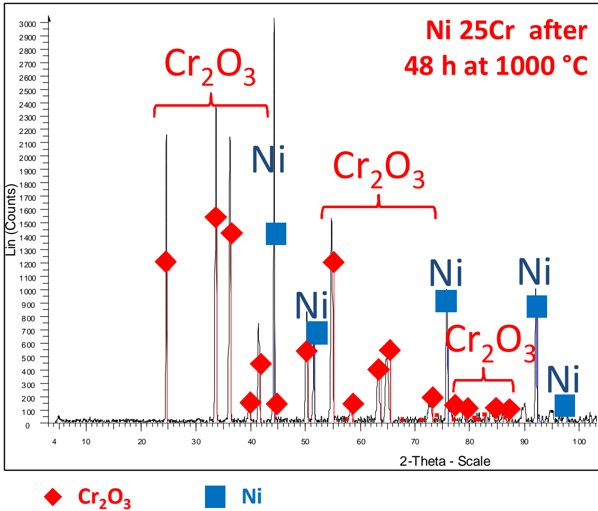
Fig. 7. Diffractogram obtained for the external oxide scale formed over the sample oxidized at 1000 °C
