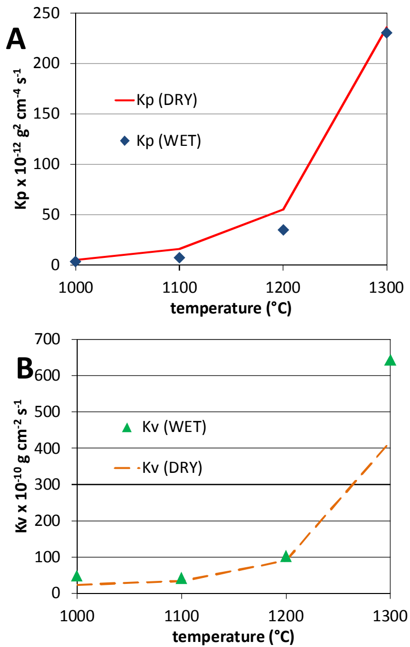
Fig. 11. Comparison of the kinetic constants of the Ni 25Cr alloy at the four temperatures between wet air and dry air ( A : K_p , B : K_v )
