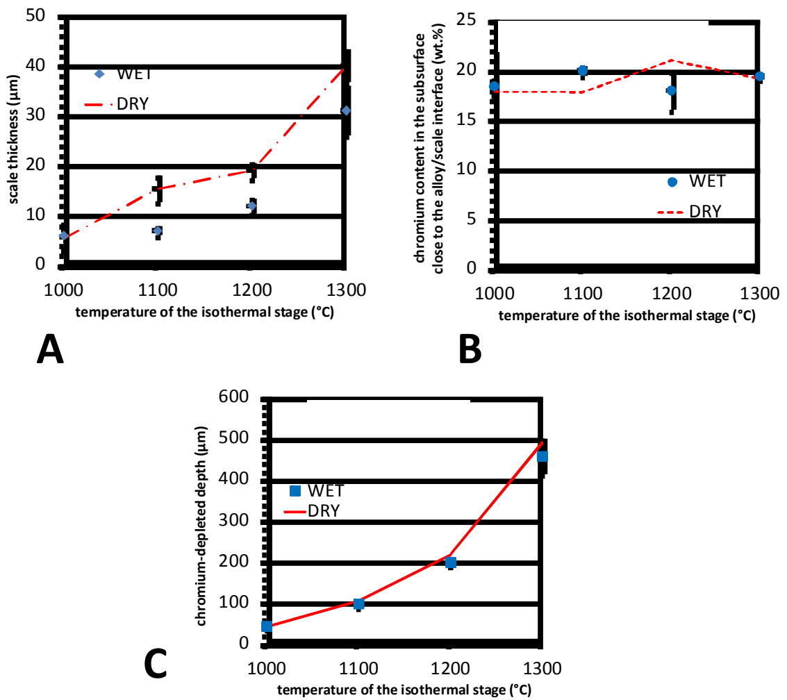
Fig. 13. Comparison of the scales' thicknesses (A), the alloy chromium contents in extreme surface (B) and the Cr-depleted depths (C) of the Ni 25Cr alloy at the four temperatures between wet air and dry air
