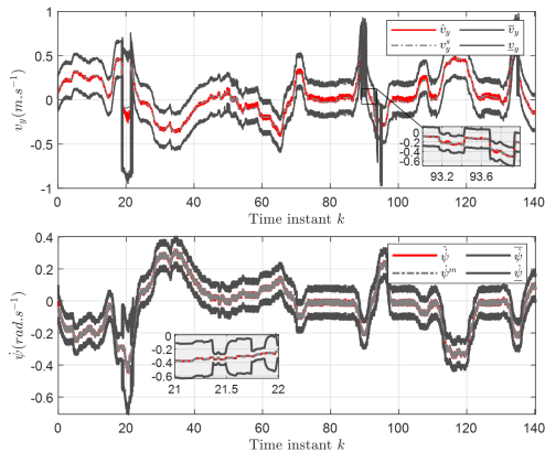
Fig. 5. Lateral velocity v_y and yaw rate \psi .
