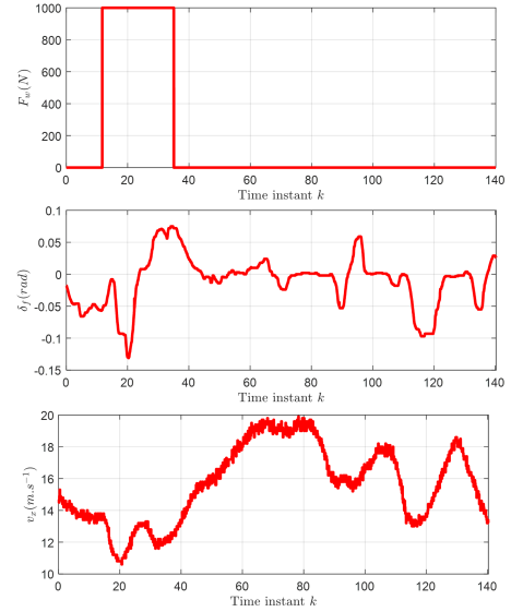
Fig. 1. Lateral wind gust input f_w , steering angle \delta_f , and longitudinal velocity v_x .
