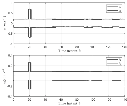
Fig. 4. Enclosure of e_1 = v_y^s - \hat{v}_y and e_2 = \psi^s - \hat{\psi} .
