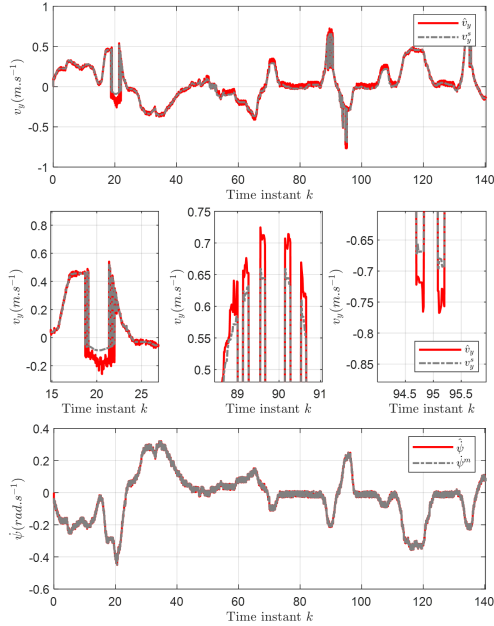
Fig. 3. Comparison of v_y^s and \hat{v}_y (first two figures) and comparison of \psi^m and \hat{\psi} .
