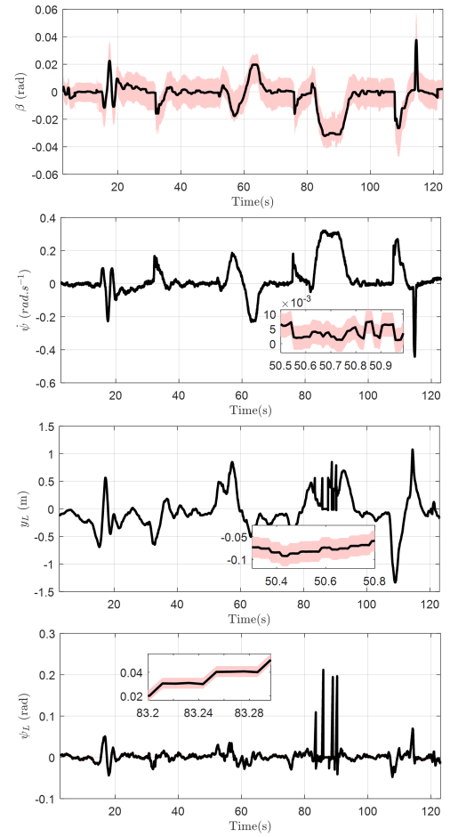
Fig. 3. Interval Estimation of vehicle side slip angle \beta , yaw rate r , angular and lateral displacements \psi_L and y_L .
