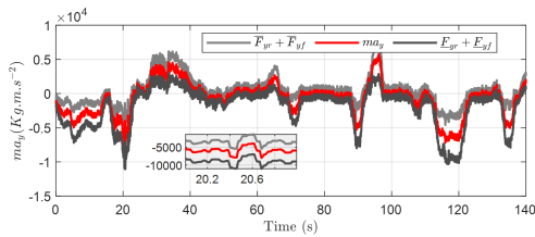
Fig. 4. Interval estimation of the signal m_{a_y} .
