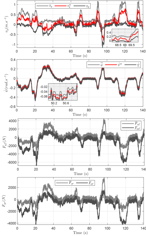
Fig. 3. Interval estimation of vehicle lateral velocity v_y , yaw rate \dot{\psi} , front and rear lateral tire force F_{yf} and F_{yr} .
