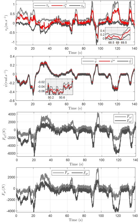
Fig. 3. Interval estimation of vehicle lateral velocity v_y , yaw rate \dot{\psi} , front and rear lateral tire force F_{yf} and F_{yr} .
