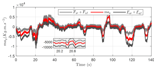
Fig. 4. Interval estimation of the signal m_{a_y} .
