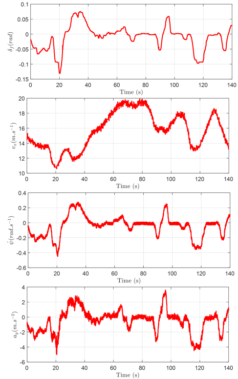
Fig. 1. Steering angle \delta_f , Longitudinal velocity v_x , Yaw rate \dot{\psi} and Lateral acceleration a_y .
