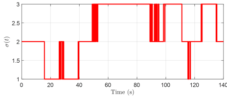
Fig. 2. Switching law \sigma(t) .
