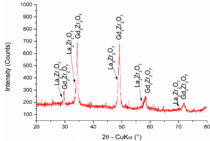
Figure 6. X-ray diffraction spectrum obtained for Nimonic with 4 layers of material (NiCrAlY/ZrO 2 -RE1/LZO/GZO).
