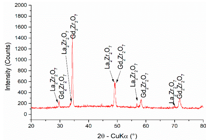
Figure 8. X-ray diffraction spectrum obtained for Nimonic with 4 layers of material (NiCrAlY/YSZ/LZO/GZO) after heat treatment at 1250 °C.
