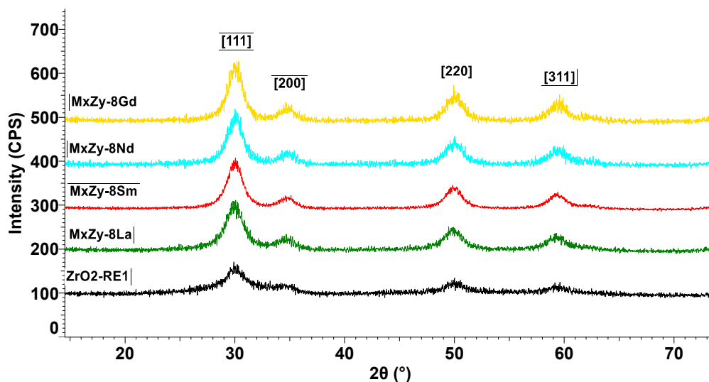
Figure 3. Diffraction spectrum for ZrO_2 -RE1, MxZy8La, MxZy8Sm, MxZy8Nd, and MxZy8Gd samples.
