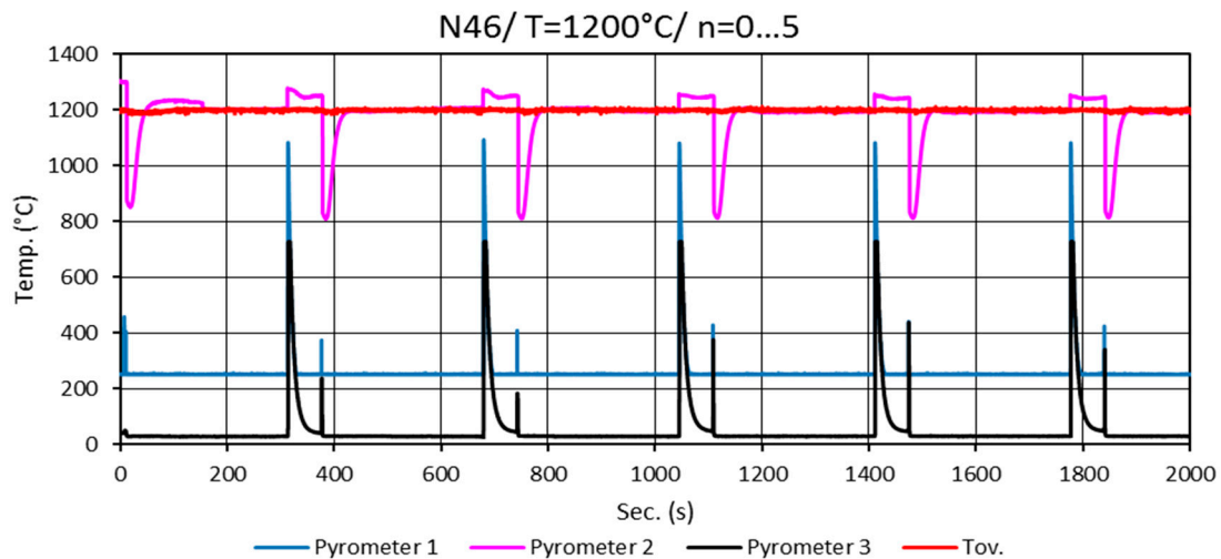
Figure 11. Thermogram for thermal shock cycles 38–43, temperature range 800–1300 °C.
