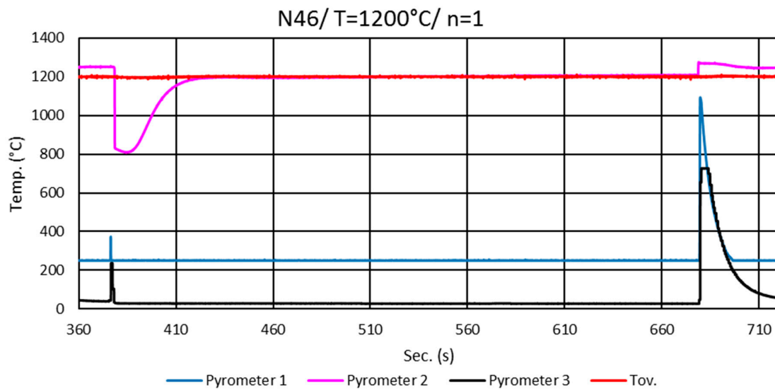
Figure 10. Thermal shock tests. The red line (TCup)—represents the recorded temperature of the oven by the Pt/PtRh thermocouple mounted inside the oven; magenta line (Pyrometer 2) represents the temperature of the sample over the heating stage during the test, which shows a peak starting from low temperature and a stabilized temperature for dwell time. The blue and black lines represent the temperature change of the sample over the cooling stage by Pyrometer 1 and Pyrometer 3, respectively.
