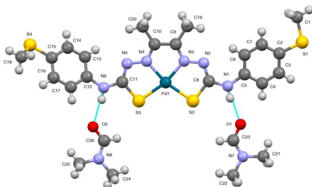
Fig. 2 X-ray crystal structure of [PdSCH 3 ] 2 ·2 DMF with atom labelling scheme and ellipsoids parameters at 50 % probability level. Selected bond lengths: Pd1-S2 2.28(10) Å, Pd1-S3 2.275(9) Å, Pd1-N3 1.98(3) Å, Pd1-N4 1.98(3) Å, N2-N3 1.36(4) Å, N2-C8 1.33(4) Å, N3-C9 1.31(4) Å, N4-N5 1.36(4) Å, N4-C10 1.31(4) Å, N5-C11 1.33(4) Å, C9-C19 1.49(4) Å, C10-C20 1.49(4) Å. Hydrogen bonds parameters: N1-H...O1 [N1-H 0.86 Å, H-O1 1.94 Å, N1...O1 2.785 Å, N1-H...O1 167.5°]; N6-H...O2 [N6-H 0.86 Å, H-O2 1.97 Å, N6...O2 2.81 Å, N6-H...O2 165.14°].
