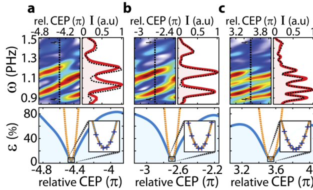
Fig. 4. Example of the extraction of the relative CEP position of a single-shot for the first 3 shots of each measurement presented in the top panels of Fig. 3(a), (b), and (c). – Top left panel: zoom in ( \pm 0.4\pi ) around the average position of -4.34\pi , -2.64\pi , and 3.56\pi in panels a, b, and c, of the harmonic spectrogram I_{\text{average}}(\omega, \text{CEP}) illustrated in Fig. 2. – Top right panel: harmonic profile in intensity of the first single-shot measurement, I_{\text{single-shot}}(\omega) , presented in the top panels of Fig. 3 in solid red line, and the profile of the spectrogram corresponding to the relative CEP positions of -4.34\pi , -2.64\pi and 3.56\pi in dashed black line (relative CEP position illustrated by the vertical dash line in the left panel). – Bottom panel: difference \varepsilon(\text{CEP}) in percentage between the single-shot harmonic profile and the spectrogram profiles as a function of the CEP calculated by Eq. (3). The sub-panel shows how the accurate single-shot relative CEP position is determined by the position of a parabolic fitting around the minimum of \varepsilon(\text{CEP}) .
