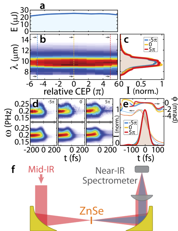
Fig. 1. Mid-IR pulse energy, panel a , and spectra, panels b and c , for different positions of the relative CEP (Eq. (2) normalized by \pi ). – d – Experimental (top panels) and reconstructed (lower panels) FROSt spectrograms for three different relative CEP positions of -5\pi , 0 , and 5\pi . – e – Retrieved temporal profiles of the mid-IR pulses in intensity, full thick lines, and phase, dash lines, and of the optical switch (see [49]) in intensity, full light lines. – f – Experimental setup for the generation and detection of high harmonics generated in a zinc selenide window (two off-axis parabolic mirrors of 50 mm focal length, and a 100 mm lens).
