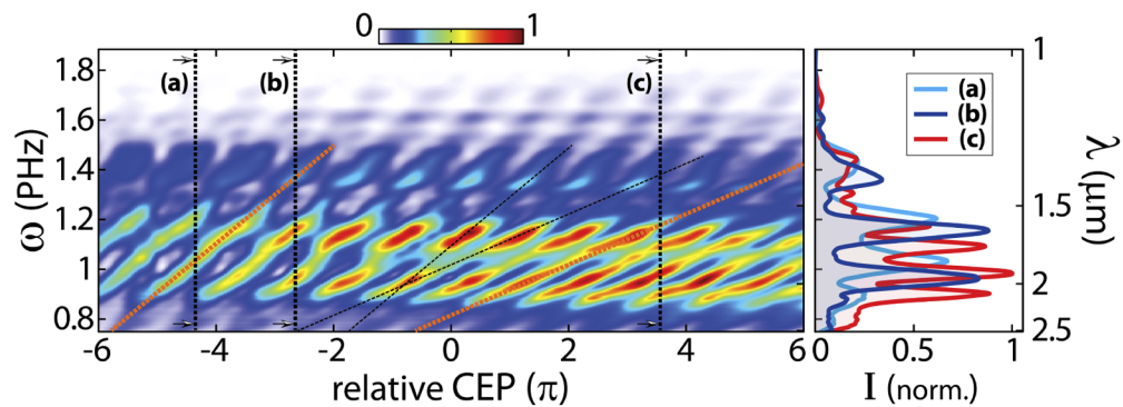
Fig. 2. Harmonic spectra measured in intensity as a function of the relative CEP of the mid-IR pulses (Eq. (2) normalized by \pi ). Oblique lines highlight the drift in wavelength of the harmonic peaks. The positions of the following three measurements of the CEP fluctuations at a fixed CEP of -4.34\pi , -2.64\pi and 3.56\pi are respectively represented with the vertical lines (a), (b), and (c). The harmonic profile at these three positions is shown on the right panel.
