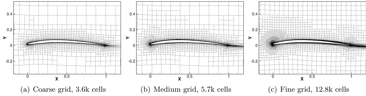
Figure 4: NACA hydrofoil computational grids.
