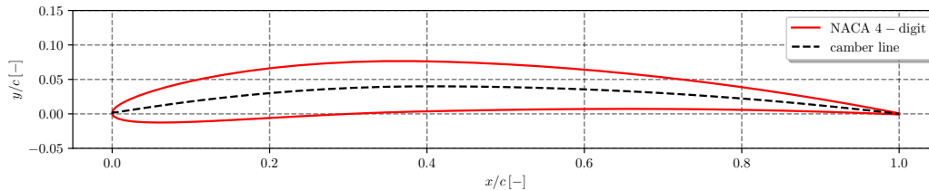
Figure 3: NACA 4-digit hydrofoil.
