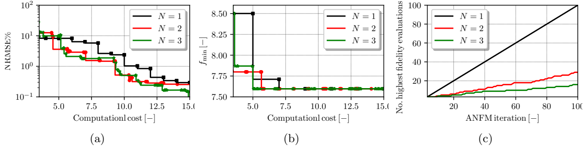
Figure 6: Analytical test problem: convergences of (a) NRMSE, (b) objective function minimum, and (c) the number of the highest-fidelity evaluations versus the sampling procedure iterations.
