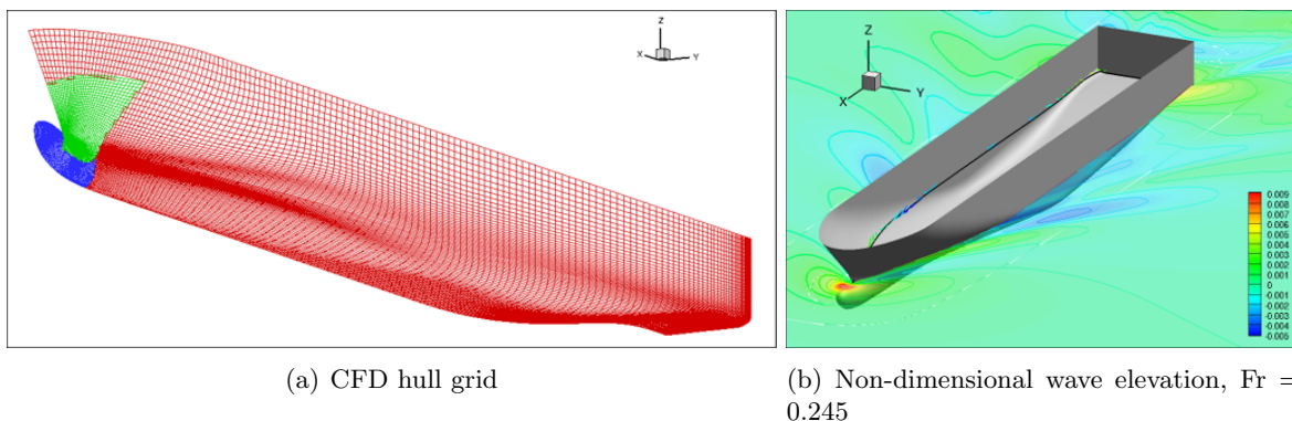
Figure 5: RoPax ferry.
