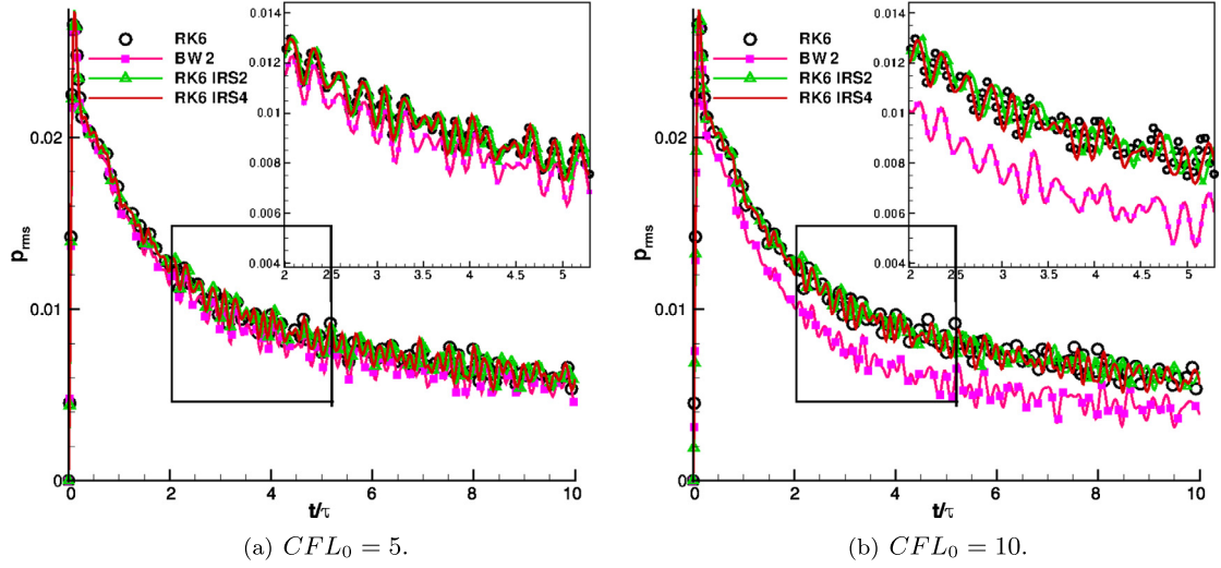
Fig. 17. HIT at M_{i0} = 2 . Comparison of the time evolution of the p_{rms} obtained with RK6 at CFL_0 = 1.7 and the RK6IRS2, RK6IRS4, and BW2 schemes with CFL_0 = 5 and 10.
