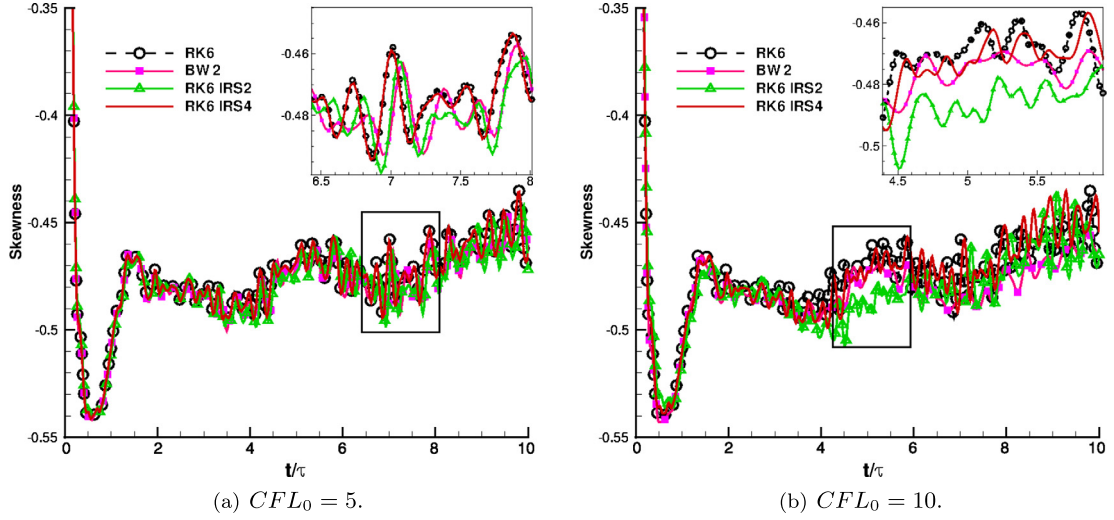
Fig. 18. HIT at M_{i0} = 2 . Comparison of the time evolution of the skewness factor of the fluctuating velocity gradient S_{v'u'} obtained with RK6 at CFL_0 = 1.7 and the RK6IRS2, RK6IRS4 and BW2 schemes at CFL_0 = 5 and 10.
