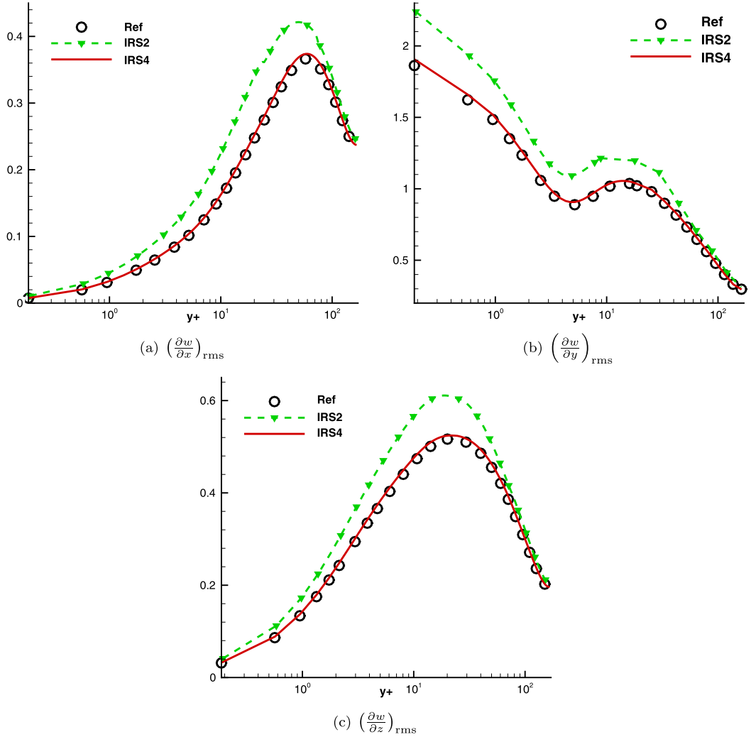
Fig. 29. Compressible turbulent channel flow. Computed (\cdot)_{rms} profiles of the velocity gradients for RK6IRS2 and RK6IRS4 at CFL_0 = 5 compared to RK6 predictions at CFL_0 = 1 (reference) [second part].
