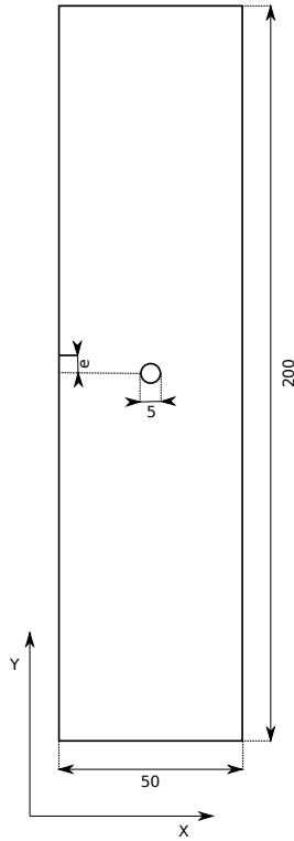
Figure 1: Sample geometry for cyclic tensile loading along Y direction parametrized by the offset e . The dimensions are in mm.
