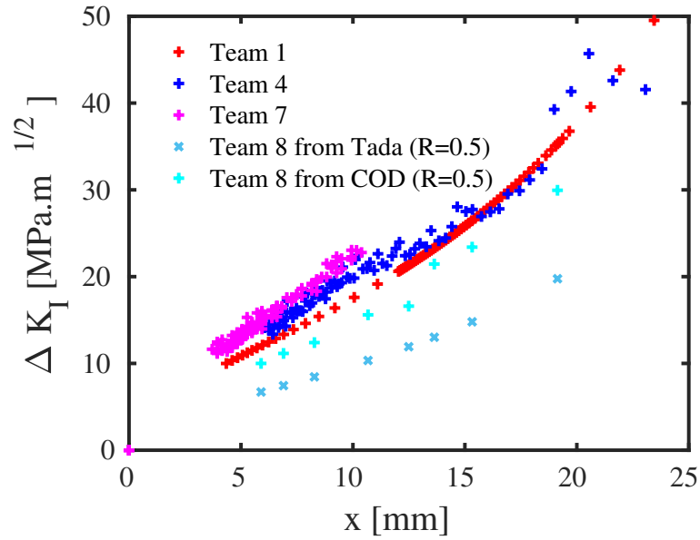
Figure 8: Aluminum alloy samples: comparison of the SIF range obtained for the 2.5 mm offset and the FF maximum force.
