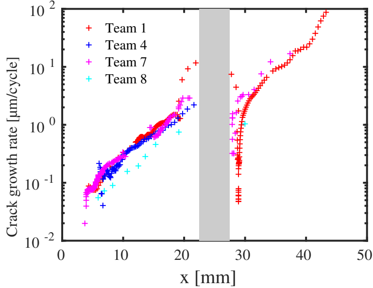
Figure 7: Aluminum alloy samples: comparison of the CGR obtained for the 2.5 mm offset and the FF maximum force. The shaded zone corresponds to the hole.
