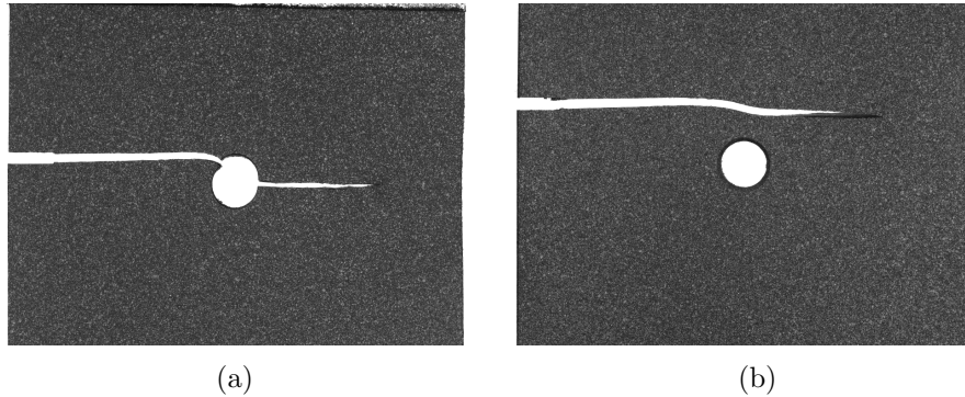
Figure 2: Comparison of the crack paths obtained for the 2.5 mm offset and the 6 mm offset (316L steel samples).
