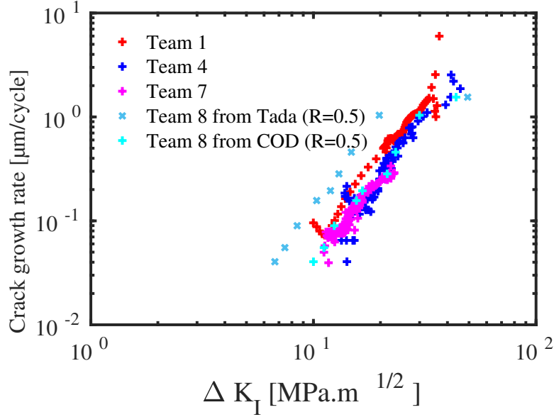
Figure 6: Aluminum alloy samples: comparison of the CGR v.s. SIF range plot obtained for the 2.5 mm offset and the FF maximum force.
