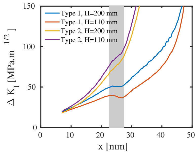
Figure 4: 316L steel samples - Comparison between the computed SIF range values ( FF ) during the propagation for type 1 (displacement imposed) and type 2 (pressure imposed) loading conditions and different grips distance H . The shaded area corresponds to the location abscissa of the hole.
