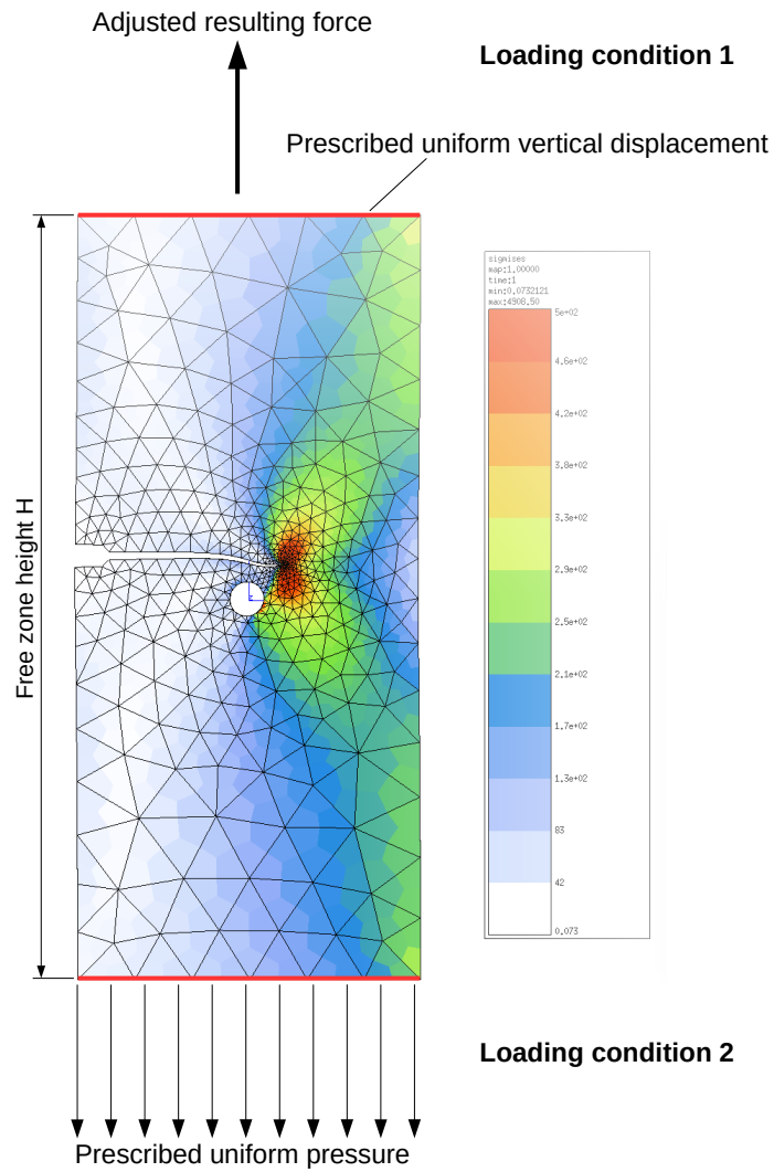
Figure 3: Representation of the two studied loading conditions, FE on a von Mises isovalues FE simulated mesh and von Mises equivalent stress contours (for illustration purpose): type (1) illustrated applied on the upper surface, type (2) illustrated applied on the lower surface.
