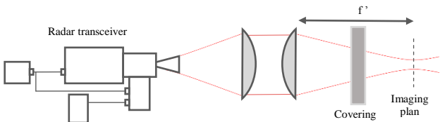
Figure 2 Optical configuration diagram for radar imaging in reflection mode with intermediate covering obstacle
