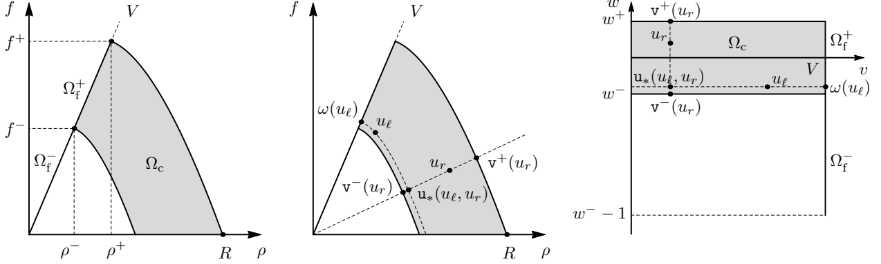
Figure 1: Notations.
