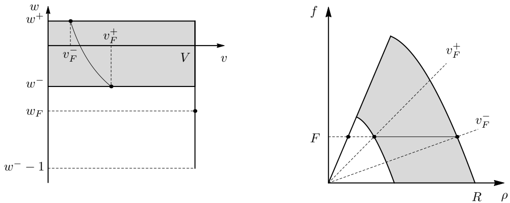
Figure 2: Geometrical meaning of w_F , v_F^{\pm} and \Xi_F in the case F \in (0, f^-) . The curve in the figure on the left is the graph of \Xi_F , which corresponds to the horizontal solid segment in the figure on the right.
