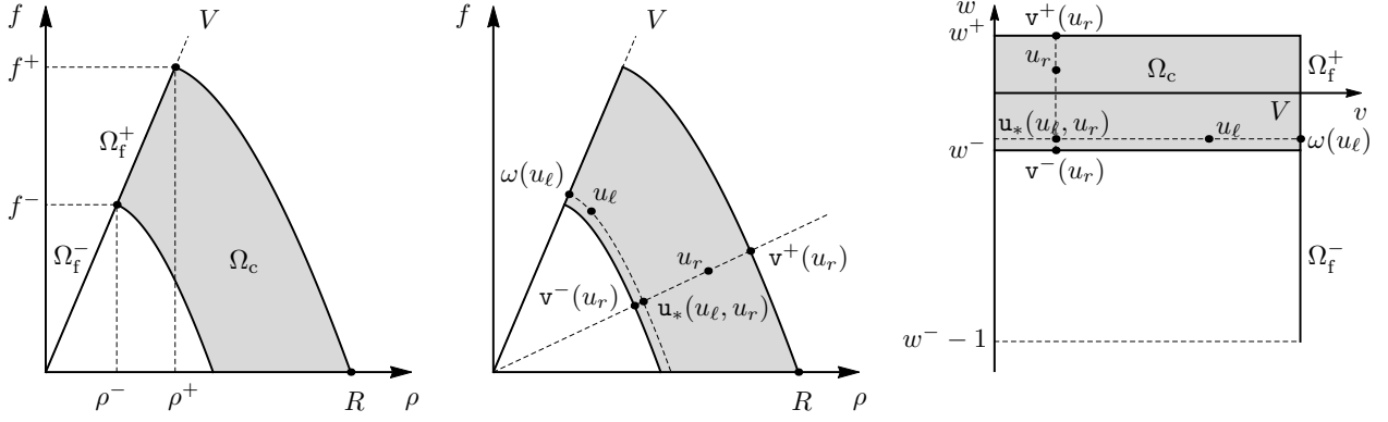
Figure 1: Notations.
