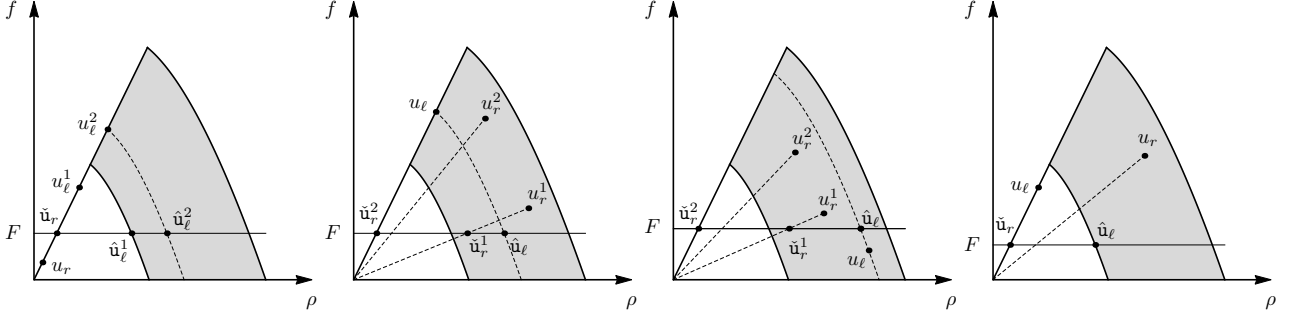
Figure 5: The selection criterion (12) for \hat{u}_\ell \doteq \hat{u}(w(u_\ell), F) and \check{u}_r \doteq \check{u}(v_r, F) exploited in Definition 3.2 in the case (u_\ell, u_r) \in \mathcal{D}_F^{\mathbf{G}} and F \in (0, f^-) . In the first picture u_\ell^1, u_\ell^2 represent the left state u_\ell^1, u_\ell^2 are the corresponding \hat{u}_\ell . Second and third pictures have analogous meaning, with u_r^1, u_r^2 and \check{u}_r^1, \check{u}_r^2 .
