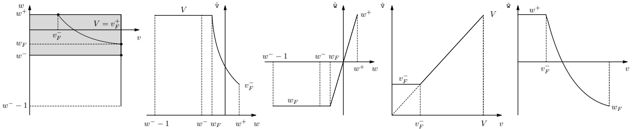
Figure 3: Geometrical meaning of \hat{u} and \check{u} defined in (12) in the case F \in (f^-, f^+) .
