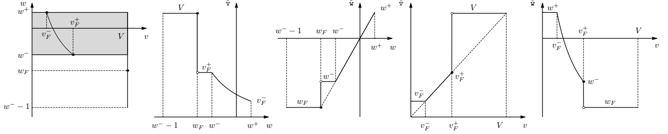
Figure 4: Geometrical meaning of \hat{u} and \tilde{u} defined in (12) in the case F \in (0, f^-) .
