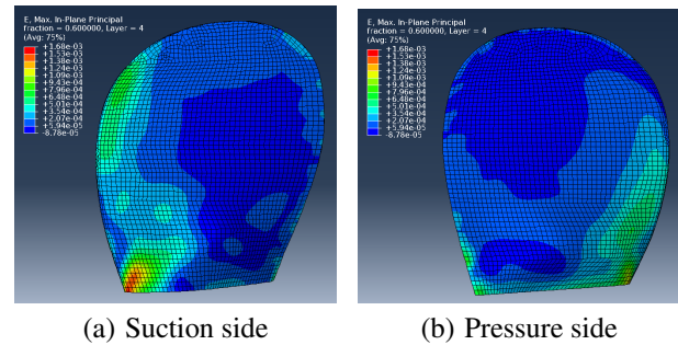
Figure 11: Instantaneous strain at the ply level of the optical fibers at 12° and 4 m/s.
