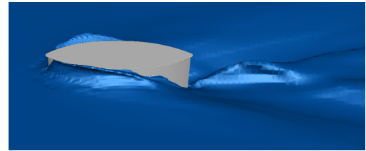
(a) Free surface elevation, top view
