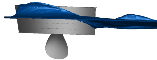
(b) Free surface elevation, side view
