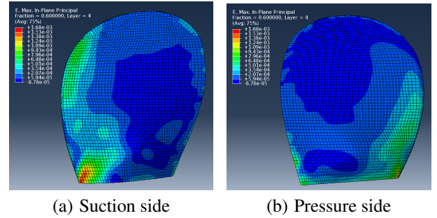
Figure 11: Instantaneous strain at the ply level of the optical fibers at 12^\circ and 4 m/s.
