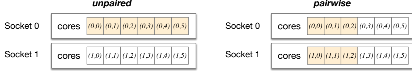
Figure 6: Example of CPU core usage for the unpaired (left) and pairwise (right) schemes when 6 cores are enabled.
