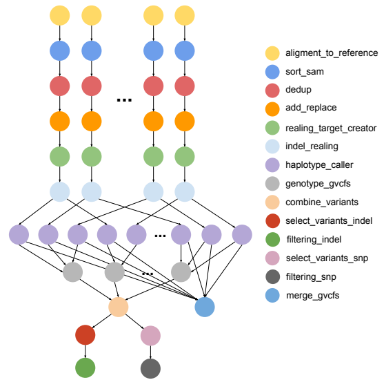
Figure 2: SoyKB workflow.
