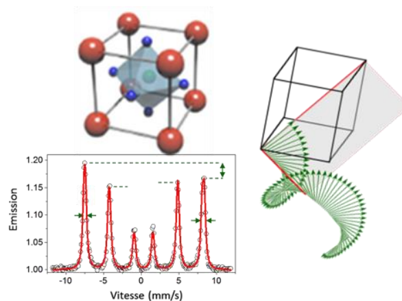
Figure 1: Mössbauer spectrum at 300 K of a 70-nm thick (001) BFO thin film grown onto GSO substrate and corresponding cycloidal spin structure derived from the fit.
