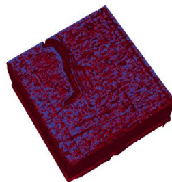
Simulation of the mechanical contact between a copper plate and a flat rigid surface
