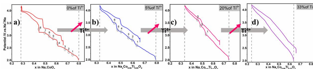
Figure 1: Galvanostatic Cycling test with Potential Limitations involving \text{Na}_x\text{Co}_{1-y}\text{Ti}_y\text{O}_2 with different titanium concentrations at sodium half-cell in the potential range 2 and 4.2V
