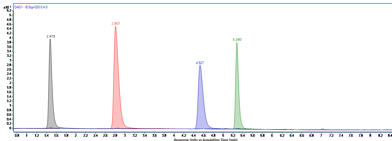
Figure 1. HPLC UV-detection chromatograms superposition of coumaroyl (red peak), caffeoyl (black peak), feruloyl (blue peak) and sinapoyl-choline (green peak)
