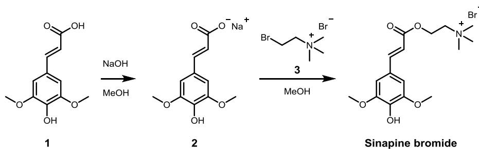
Scheme 2. Synthetic strategy to sinapine from Wathelet et al. [9a]
