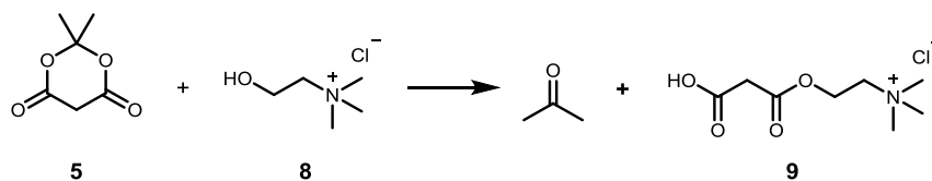
Scheme 4. Formation of the choline chloride malonate monoester ( 9 )
