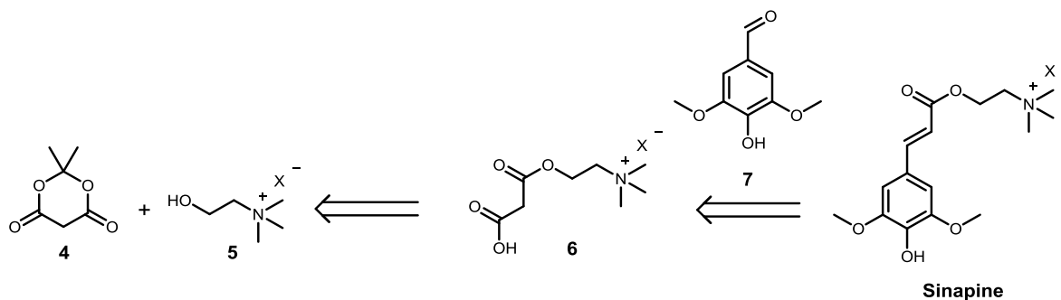
Scheme 3. Retrosynthetic approach for the synthesis of sinapine
