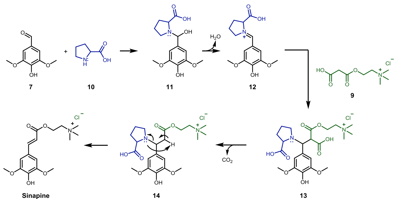
Scheme 5. Proline-mediated Knoevenagel-Doebner condensation's mechanism
