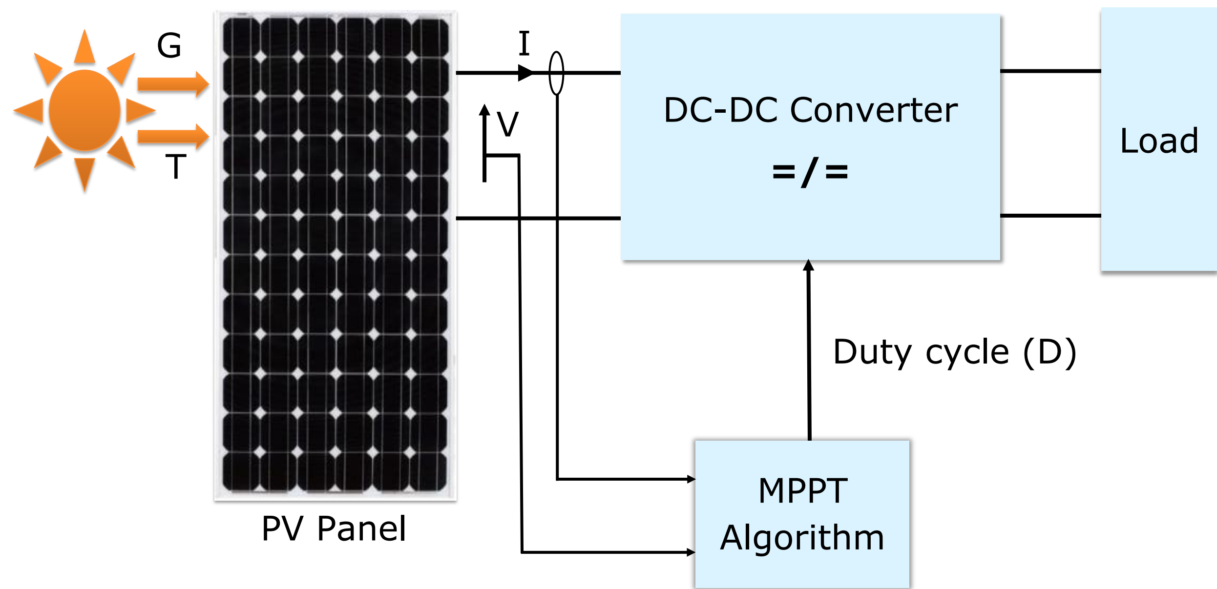
Figure 1 : PV system with maximum power point tracking (MPPT)
