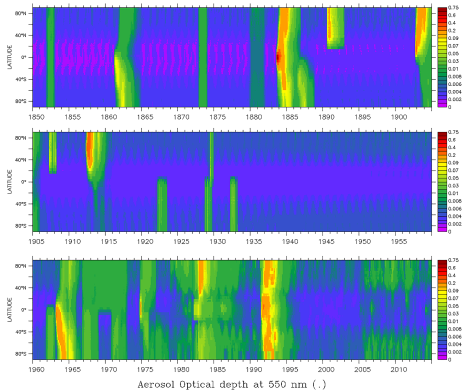
Figure 12. Latitude-time variations in stratospheric aerosol optical depth at 550 nm as diagnosed in IPSL-CM6A-LR after interpolation of the original data set onto the model grid and removal of the tropospheric contribution based on the model tropopause height detection. The 1850–2015 period is shown as split in three different panels.
