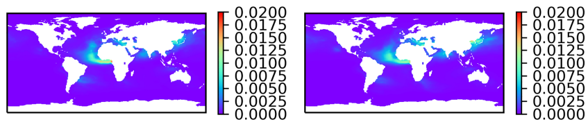
Figure 14. Iron deposition rate (in \text{g}\cdot\text{m}^{-2}\cdot\text{year}^{-1} ) at the surface as prescribed in IPSL-CM6A-LR, averaged over decades 1850–1859 (left) and 2000–2009 (right).
