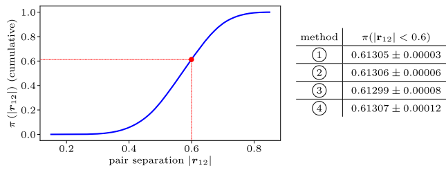
Fig. 14. Cumulative histogram of the pair separation |r_{12}| (nearest image) for two charges in a periodic three-dimensional cubic simulation box with periodic boundary conditions ( \beta c_1 c_2 = 2 , L = 1 ). ①: Reversible Markov-chain Monte Carlo (see [21, Fig. 8]) ②: Method of Section 5.1.1 ③: Method of Section 5.1.2 ④: Method of Section 5.1.3, each with standard errors for \pi(|r_{12}| < 0.6) .
