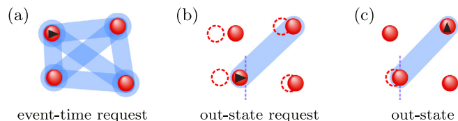
Fig. 9. Set of pseudo-factors realized by the end-of-chain event handler. (a) Set of end-of-chain pair pseudo-factors for four point masses coupling the final active unit of the old chain and the beginning active unit of the new chain. (b) At the event time, the realized pseudo-factor with the incoming active unit and the outgoing unit is known. (c) A new event chain is started. The outgoing active unit is shown.
