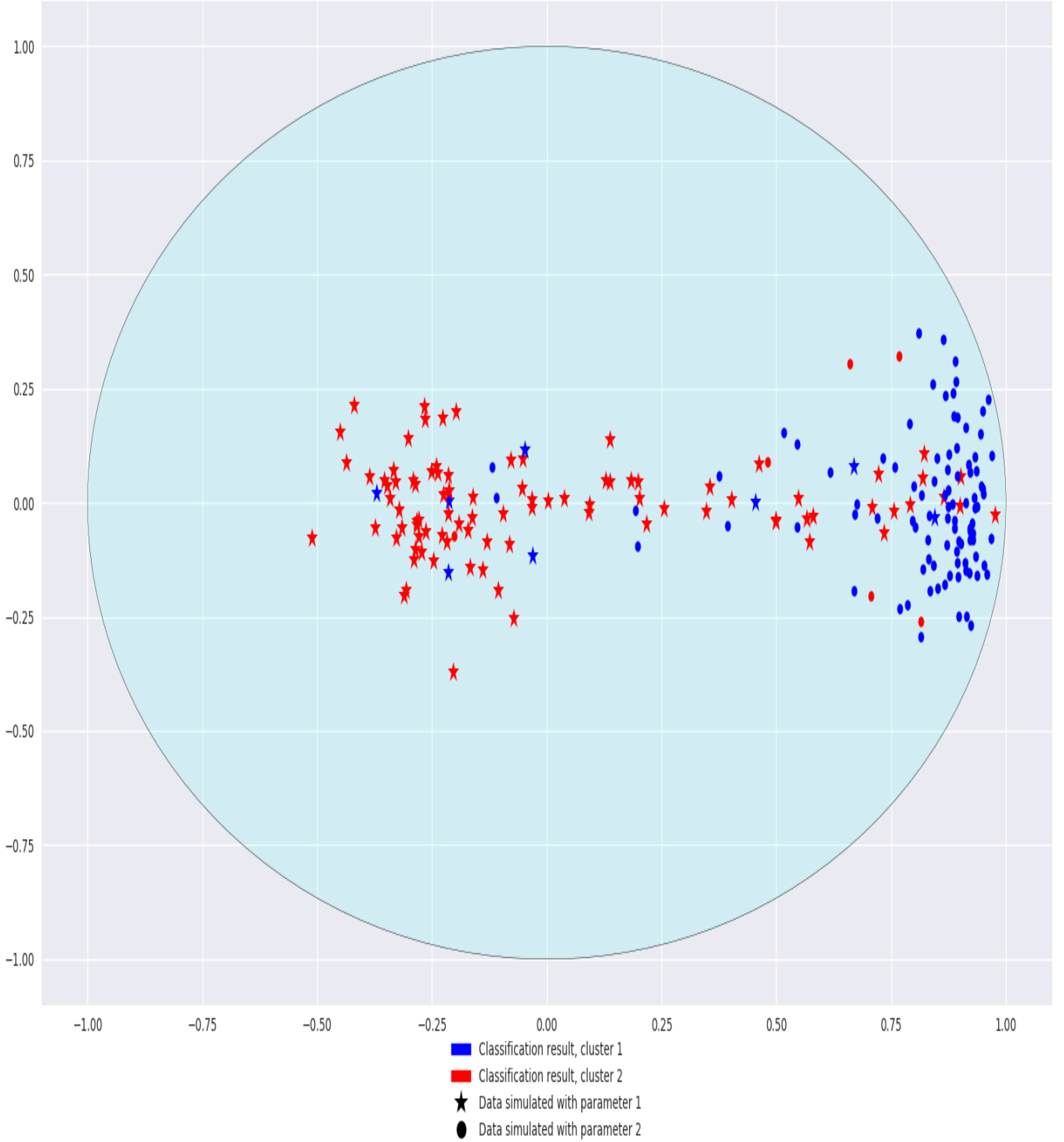
Figure 2: Second coefficient of reflection, k-means on \mathbb{D}^{n-1} , Kähler metric
