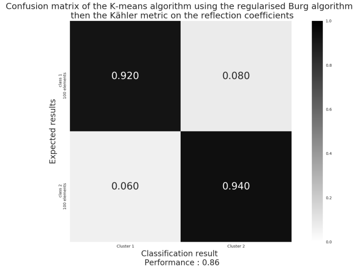
Figure 3: Confusion matrix, k-means on \mathbb{D}^{n-1} , Kähler metric
