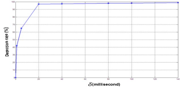
Fig. 4. Passive attacks' detection rate versus \delta
