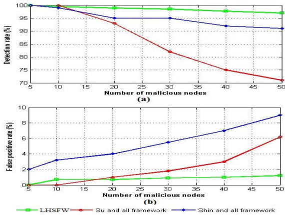
Fig. 5. LHSFW performances in terms of: (a) Detection rate, (b) False positive rate
