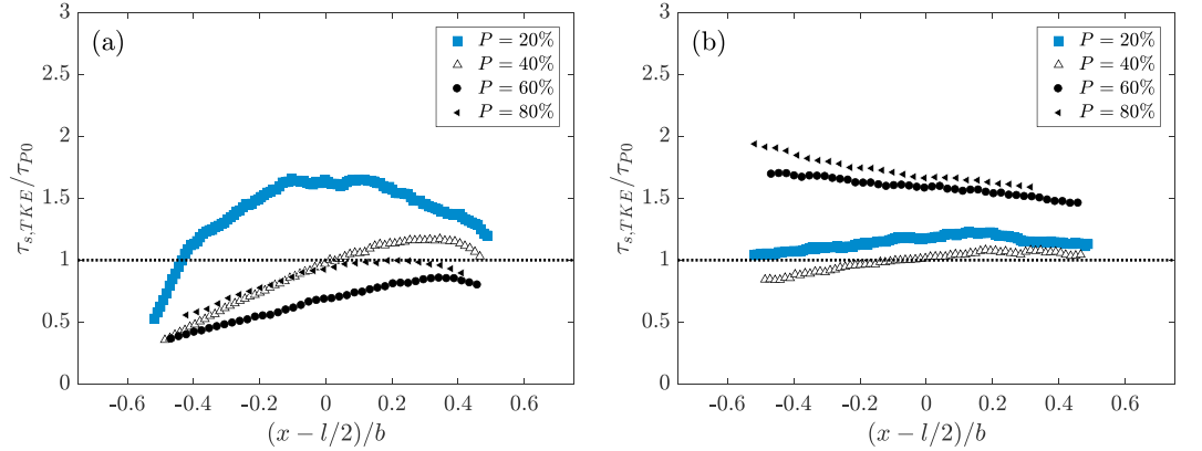
Figure 10. Horizontal profiles of fine-sediment shear stress \tau_{s,TKE} estimated with the turbulent kinetic energy between the spherical caps and normalized with the reference shear stress \tau_{P0} for all protrusion P \geq 20\% for Re_D = 27, 700 in (a) plane C and (b) plane A (Figure 1c).
