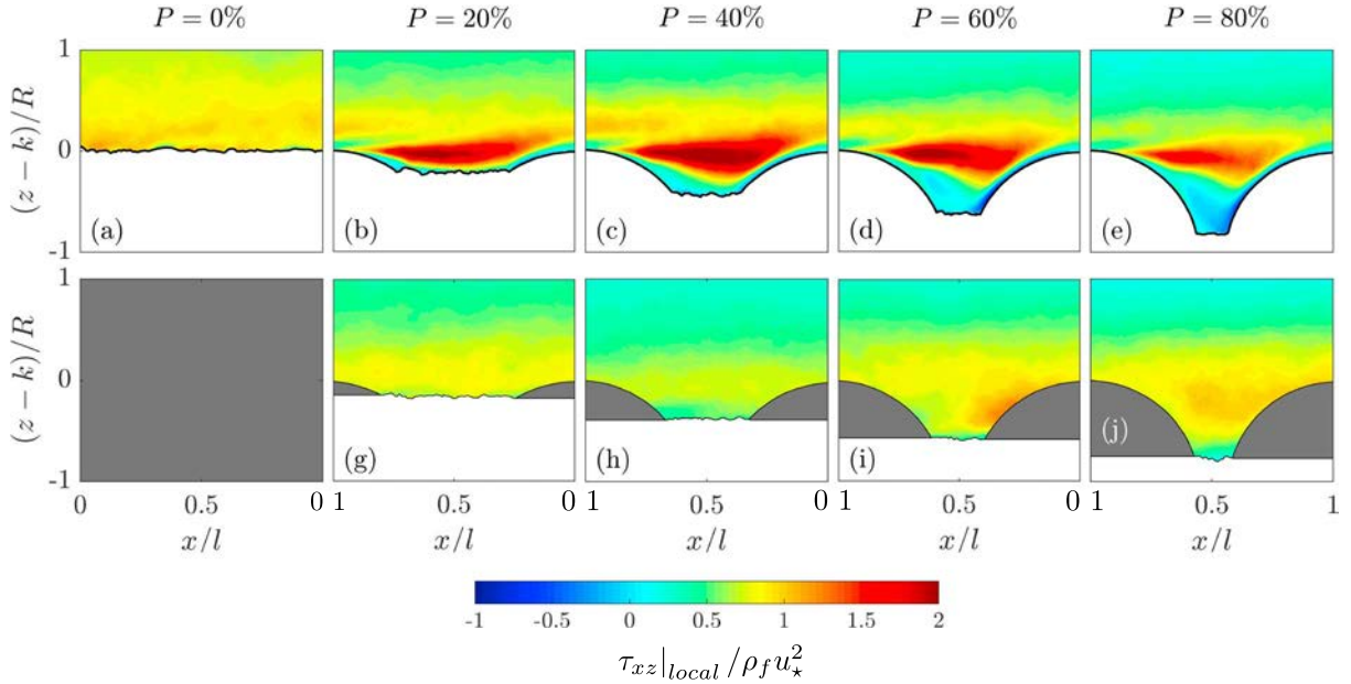
Figure 3. Dimensionless local shear stress \tau_{xz}|_{local}/\rho_f u_*^2 for Re_D = 27,700 for the different protrusion levels. (a–e) Measurements in plane C. (g–j) Measurements in plane A. Gray areas are regions hidden from particle image velocimetry measurements.
