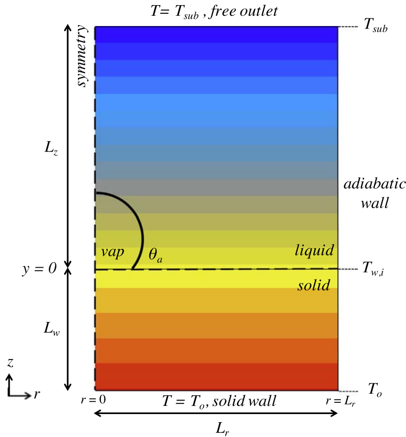
Fig. 2. Computational domain, initial conditions (temperature field and initial vapour seed) and boundary conditions. Size of the seed not in scale.
