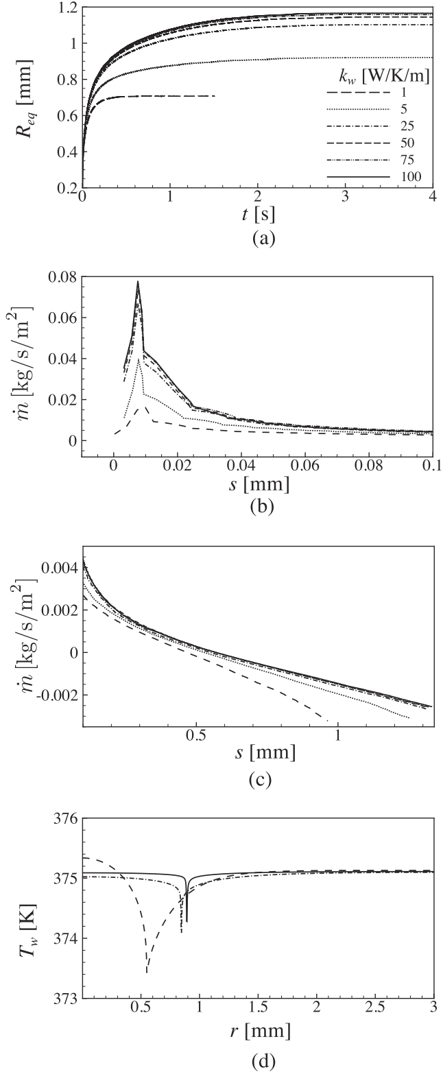
Fig. 5. Numerical results for Ja_c/Ja_e = 5 and \theta_a = 50^\circ for different k_w . (a) Equivalent diameter of the bubble against time. (b) and (c) \dot{m} distribution along the bubble interface in stationary conditions. (d) T_w distribution ( y=0 ) in stationary conditions.
