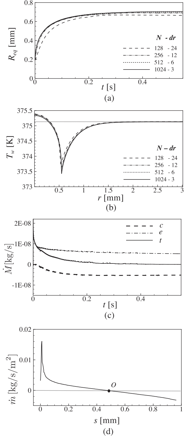
Fig. 3. Results for Ja_c/Ja_e = 5 and \theta_0 = 50^\circ . Temporal evolutions of the equivalent vapour radius (a) and spatial distribution of temperature along the wall ( z = 0 ) (b) for different grids ( dr in \mu\text{m} ). Temporal evolution of the phase change mass flow rate (c) and distribution of the specific phase change mass flow rate along the bubble interface s (curvilinear abscissa) (d).
